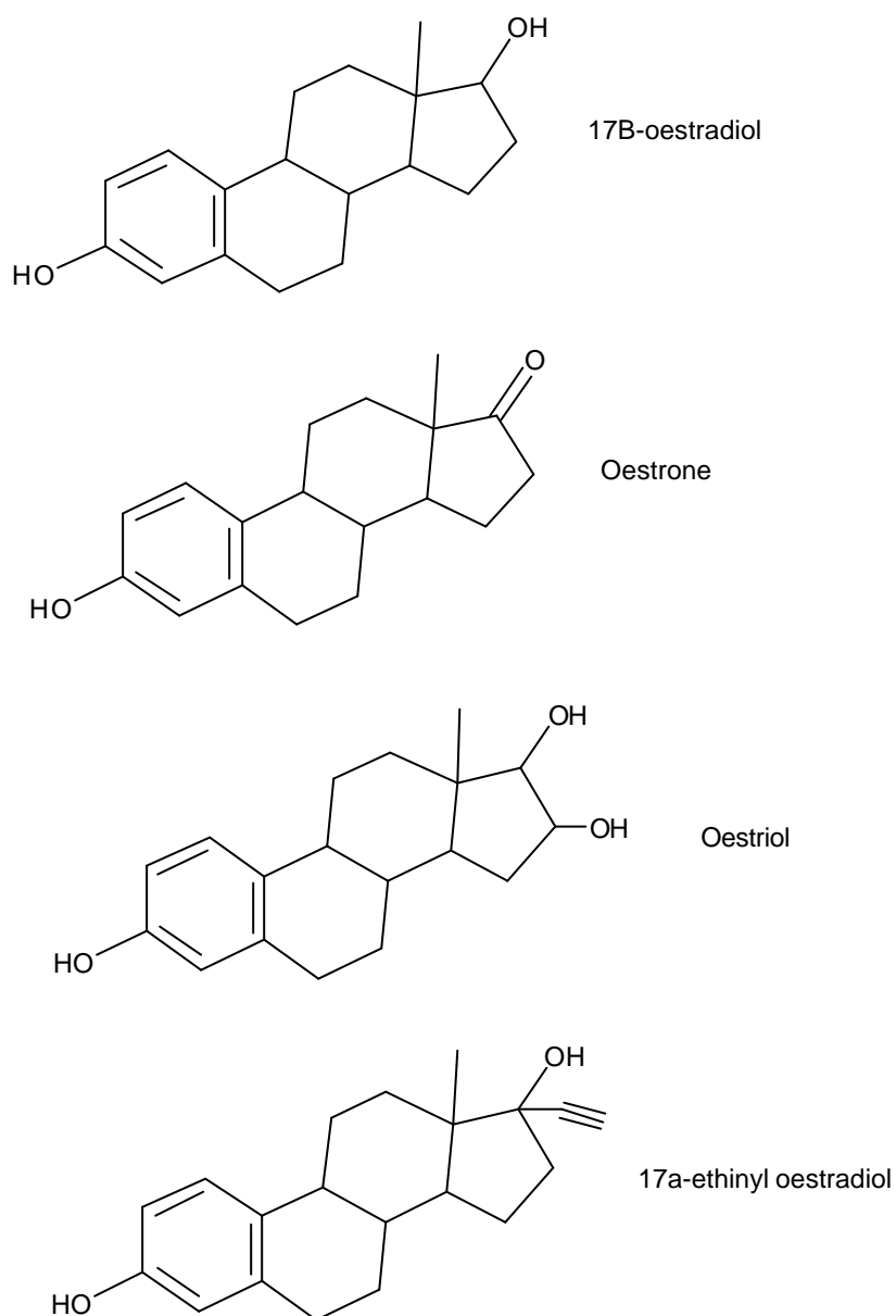
Figure 2.1 Chemical structures of the main steroid oestrogens
